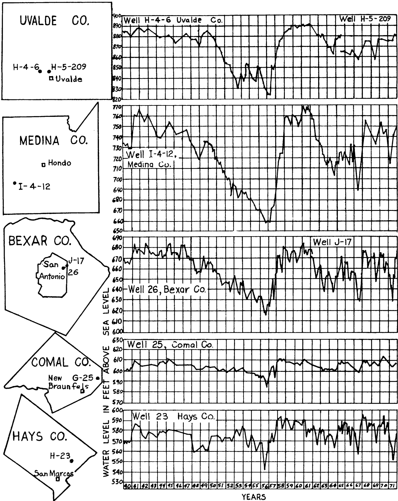
Figure 10 Hydrographs of Representative Wells in the Edwards (Balcones Fault Zone) Aquifer, 1940-1971 (Modified From Garza, 1966)
